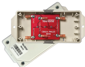
auxiliary input module provides 2 inputs capable of monitoring devices such as door contacts, security panel outputs, and more
